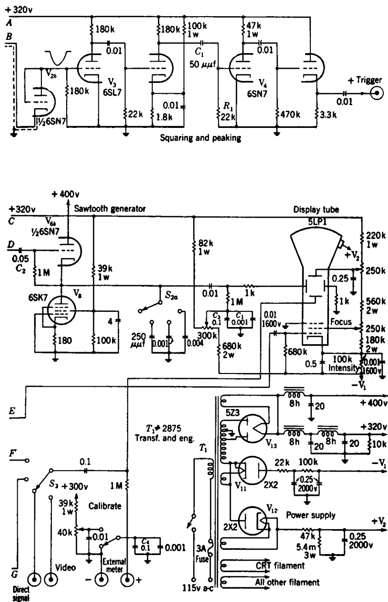
Fig. 7-4b.—Schematic circuit diagram of P-4 synchroscope (continued).
